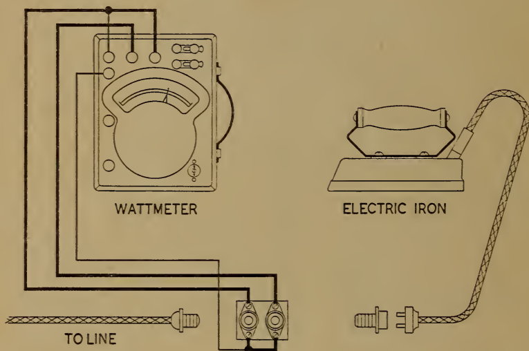
FIG. 17.—BEALS' WATTMETER METHOD. (Reproduced from Connection Chart.)
